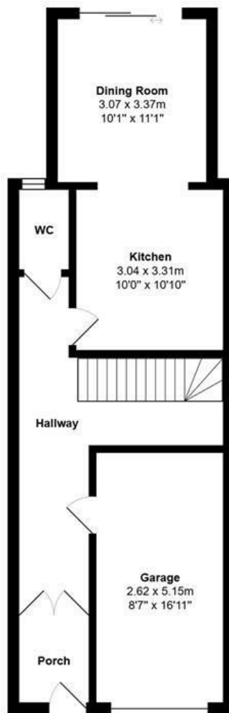
Ground Floor Area: 55.5 m 2 ... 598 ft 2
