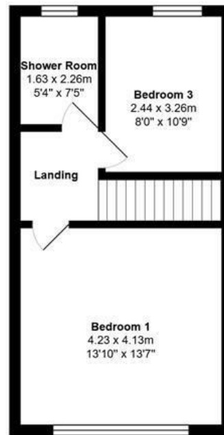
Second Floor Area: 36.3 m 2 ... 390 ft 2
